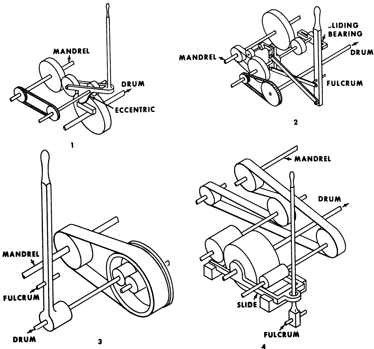
Figure 8-5. Friction-belt-pulley feed works.
